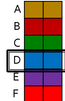
Embeddings H_1
