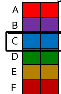
Embeddings H_2
